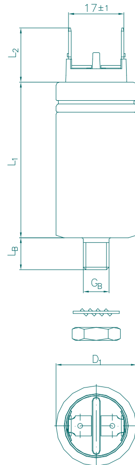
outline drawing
